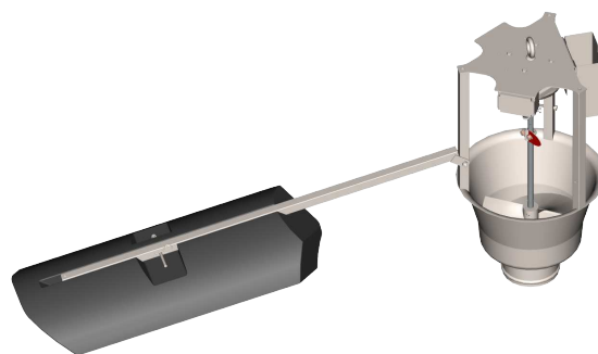
Fig 3: Float Arm Assembly
